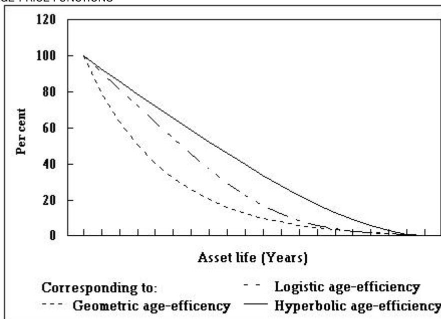
Graph 14.2 AGE-PRICE FUNCTIONS
